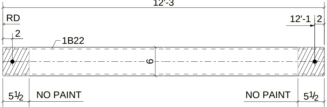
ONE - HSS GIRT - 1B22
